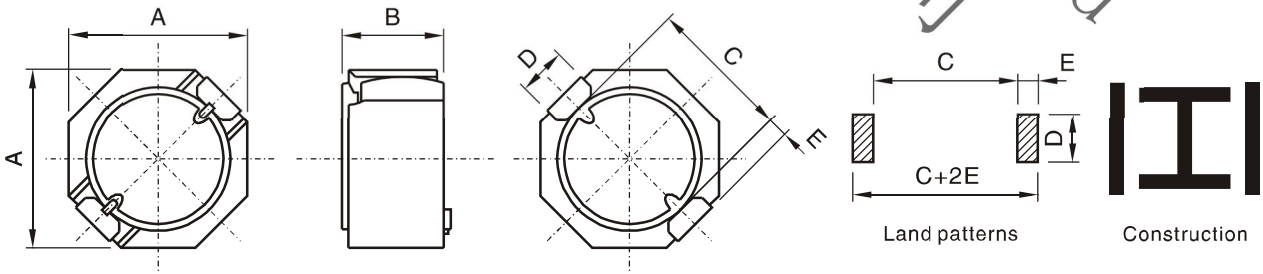
DIMENSIONS IN:mm
