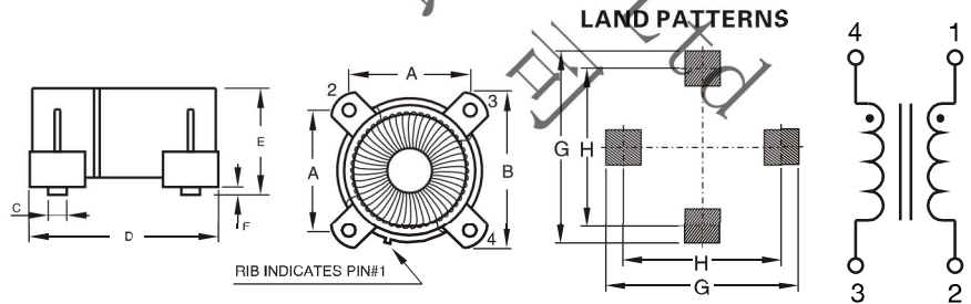
DIMENSIONS IN:mm
