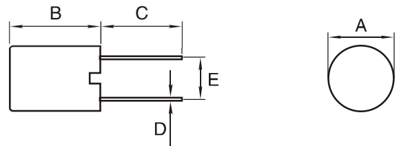
DIMENSIONS IN:mm
